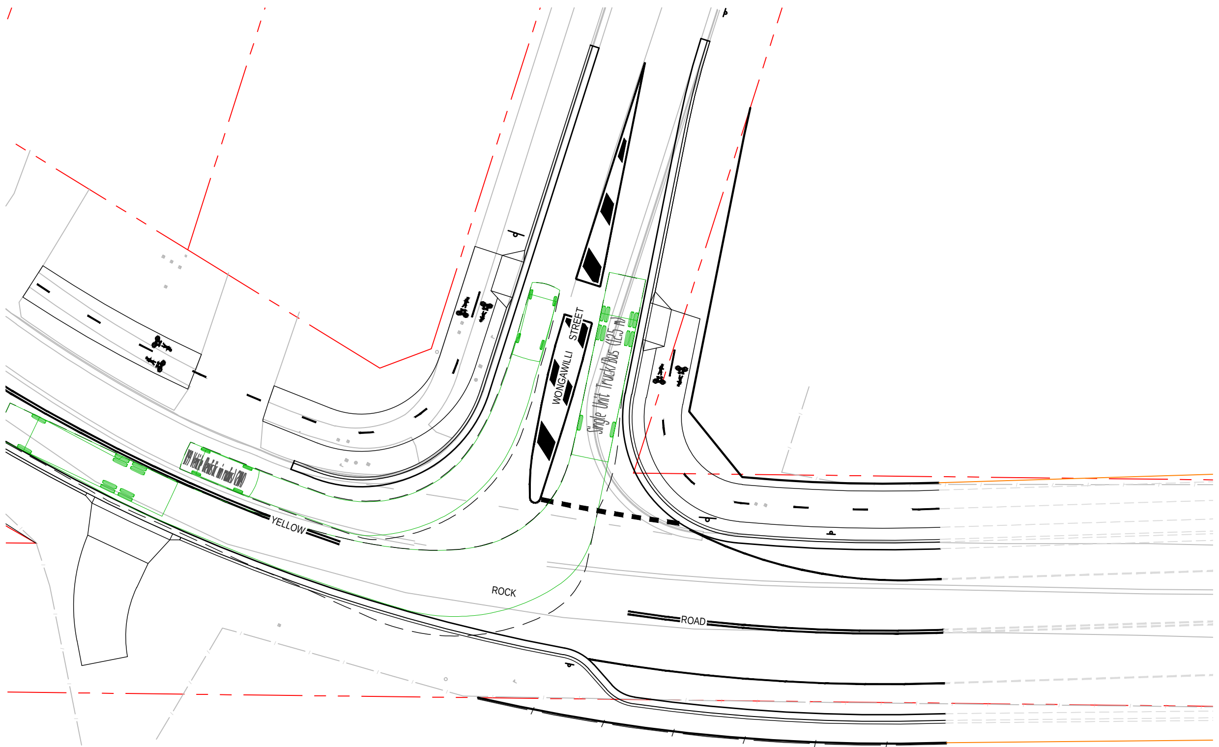
KR 03 & KR 04 TURNING PATH PLAN SCALE 1:250
