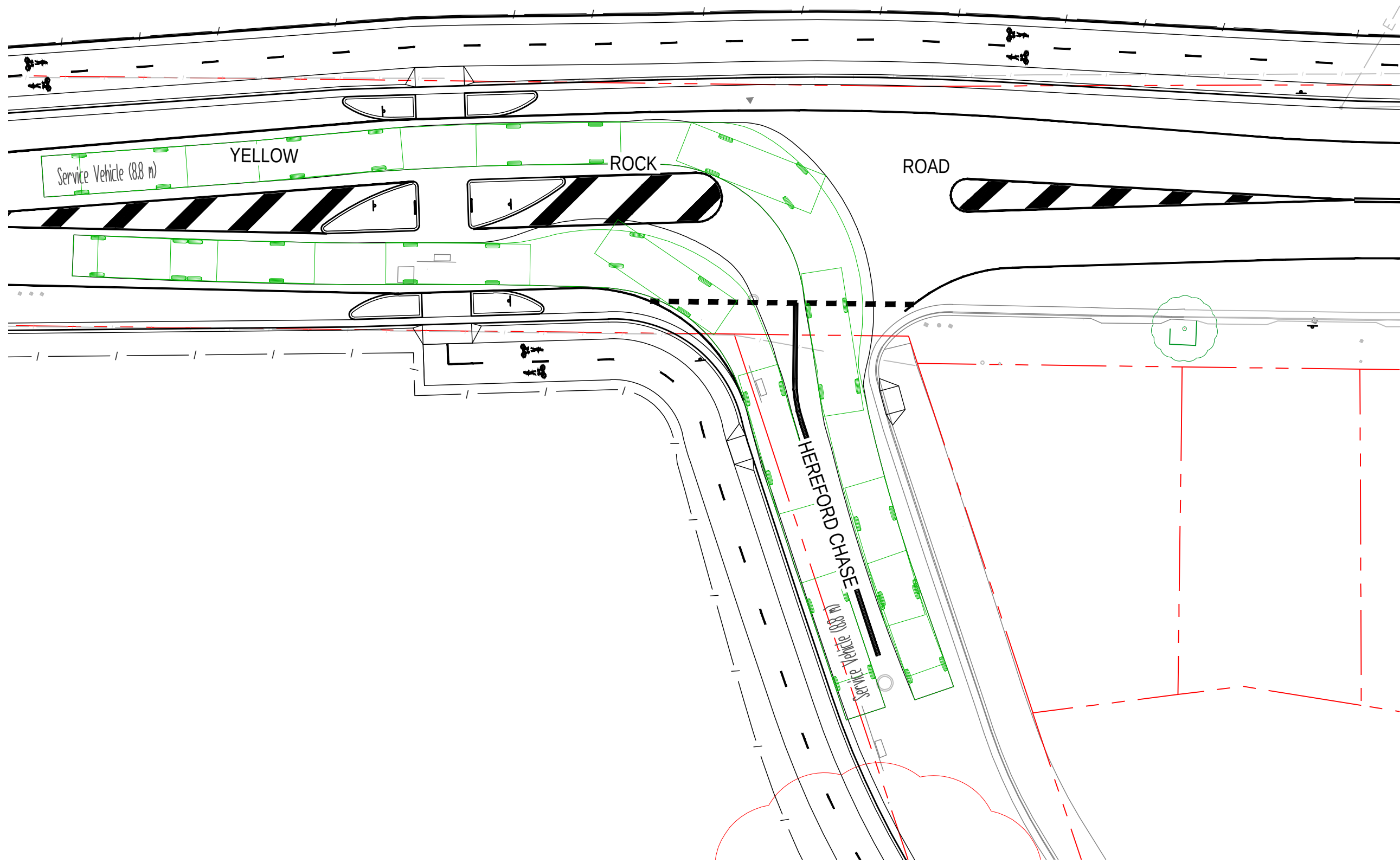
KR 05 & KR 06 TURNING PATH PLAN 2 SCALE 1:250
