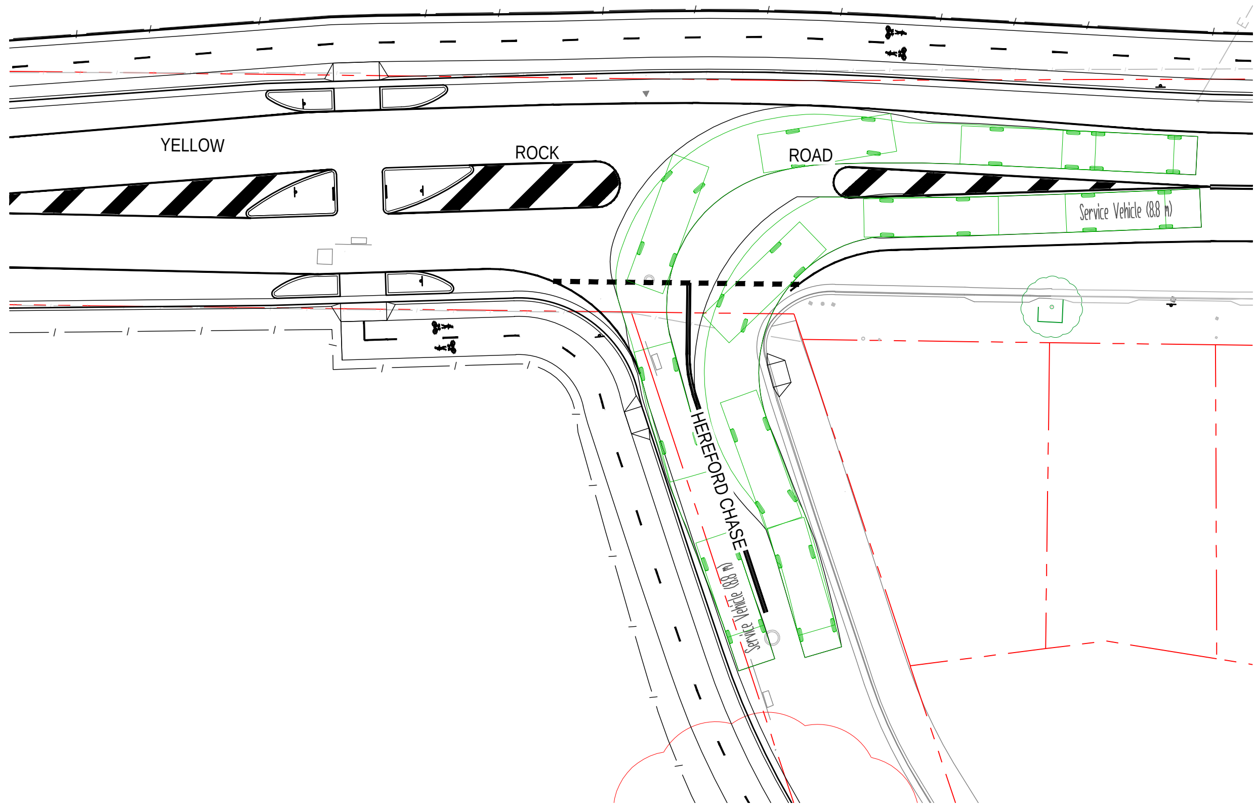
KR 05 & KR 06 TURNING PATH PLAN 1 SCALE 1:250
